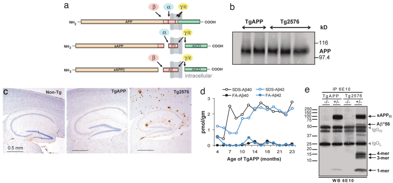
Fig. 1. TgAPP mice do not accumulate A \beta or amyloid plaques with age. (a) Schematic diagram of APP, a transmembrane protein, and its major proteolytic products. Cleavage of APP by \alpha -, \beta -, \gamma -, and \epsilon -secretases produces secreted amino-terminal fragments, carboxyl-terminal polypeptides, and A \beta . (b) Western blot analysis of whole-brain homogenates probed with 6E10 antibodies shows \approx 6 units of wild-type human APP in TgAPP brain, similar to the level of mutated human APP expressed in Tg2576 mice. (c) Immunohistology performed with 4G8 antibodies on hippocampal and overlying cortical brain areas shows no amyloid plaques in 19-month non-Tg or TgAPP mice, in contrast to abundant plaques in 18-month Tg2576 mice. (d) ELISAs of SDS-soluble (SDS) and SDS-insoluble, formic acid-soluble (FA) A \beta 40 and A \beta 42 species show low levels throughout life. (e) Immunoprecipitation (IP) with 6E10 antibodies and Western blotting (WB) with 6E10 antibodies of soluble extracellular-enriched brain extracts from 12-month TgAPP (+/-) and non-Tg (-/-) littermates and 13-month Tg2576 and non-Tg littermates shows A \beta *56 only in the Tg2576 mouse. IgG H and IgG L are the heavy and light chains of immunoglobulins, respectively. Arrows indicate bands comigrating with tetramers (4-mer), trimers (3-mer), and monomers (1-mer) of A \beta . Bars are means; error bars are SEM.
